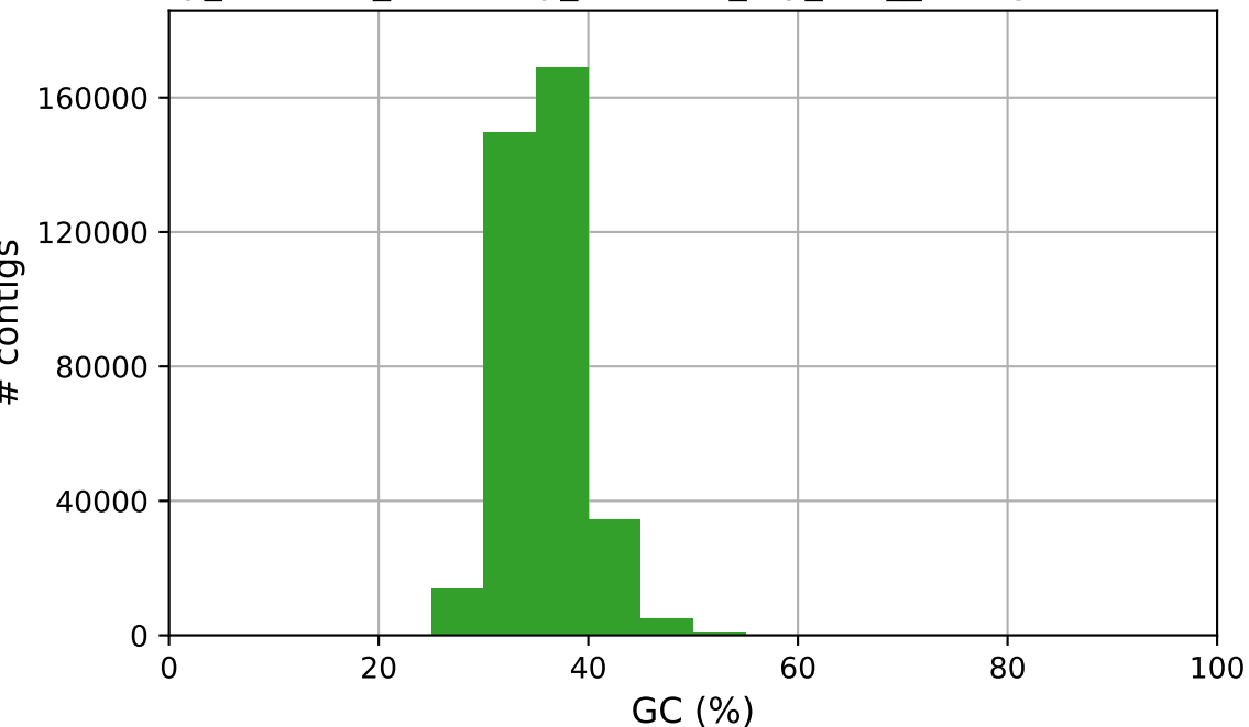
Oly_Platanus_Assembly_Kmer-22_Oly_Out__contig GC content
