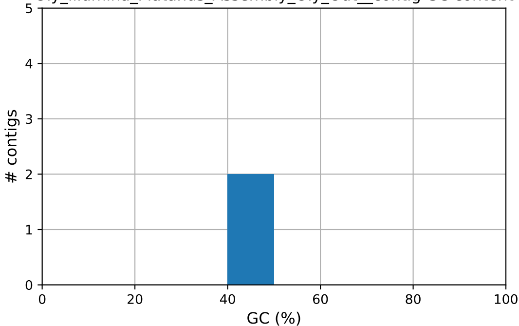
Oly_Illumina_Platanus_Assembly_Oly_Out_contig GC content
