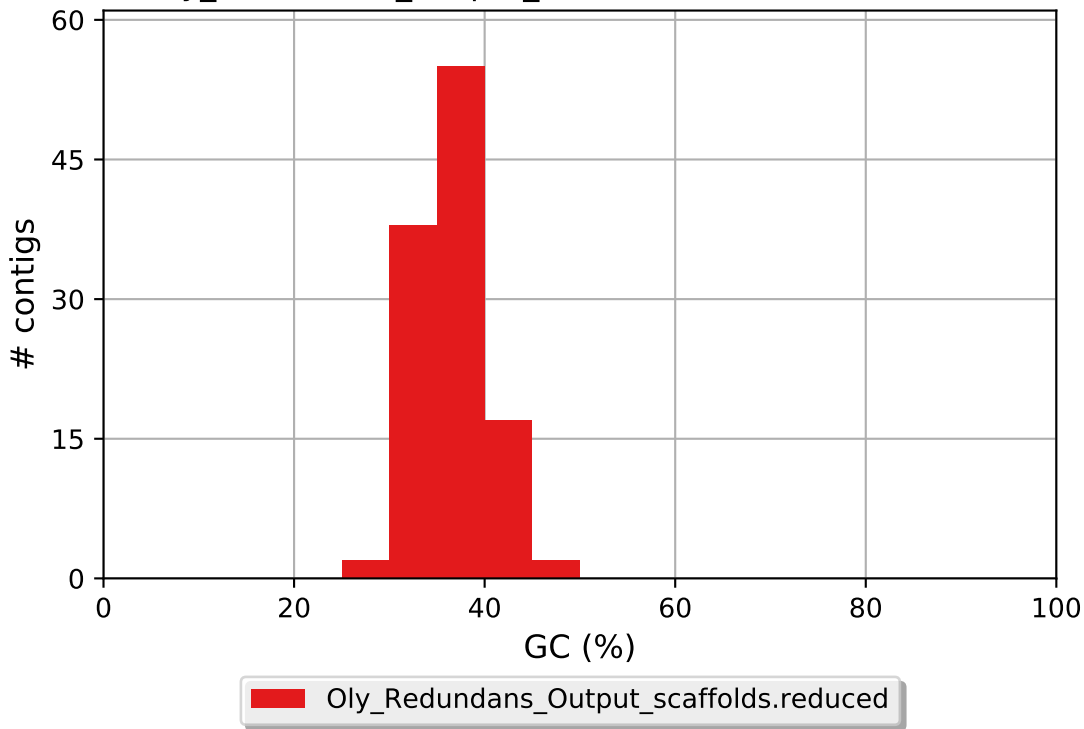
Oly_Redundans_Output_scaffolds.reduced GC content
