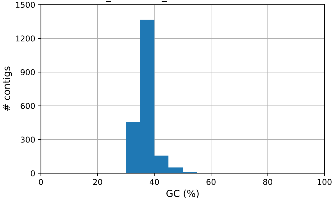
20171005_redundans_scaffolds.reduced GC content
