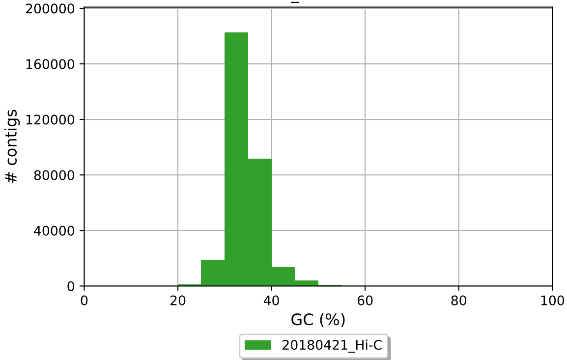
20180421_Hi-C GC content
