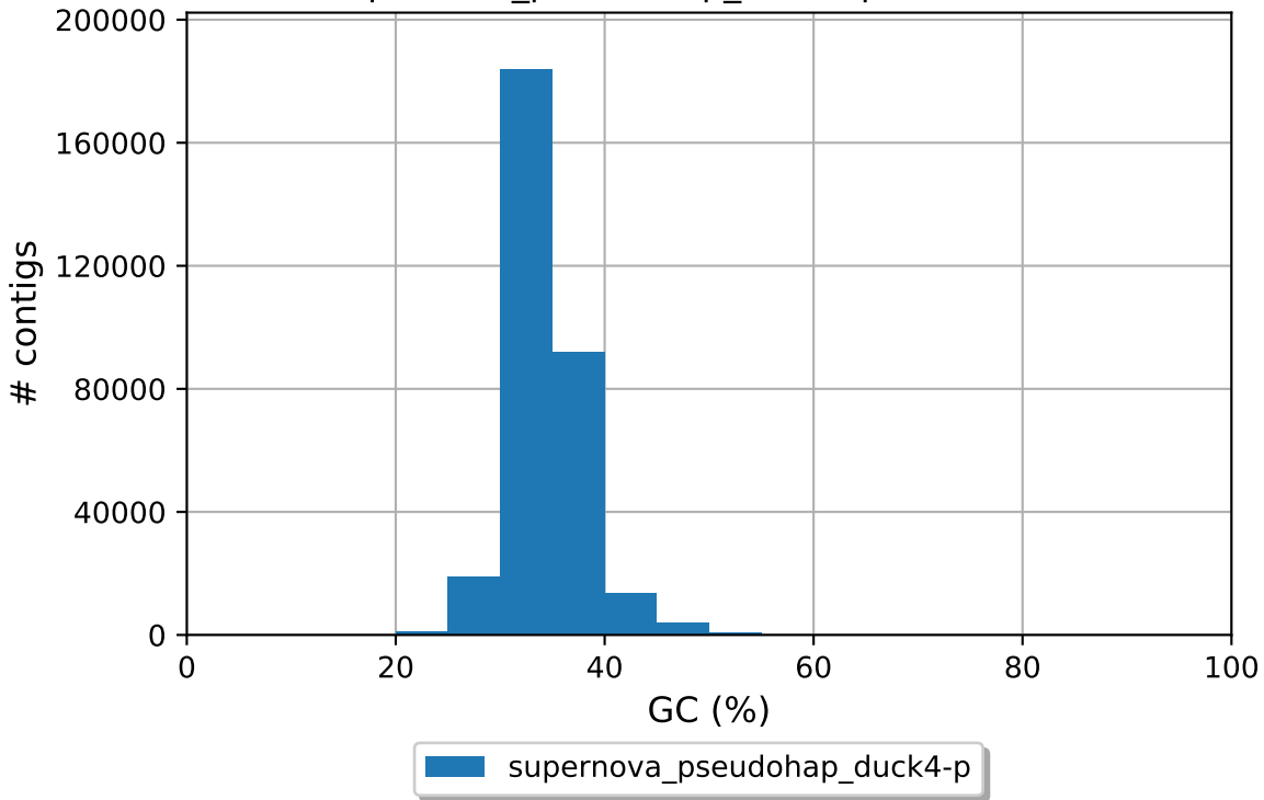
supernova_pseudohap_duck4-p GC content
