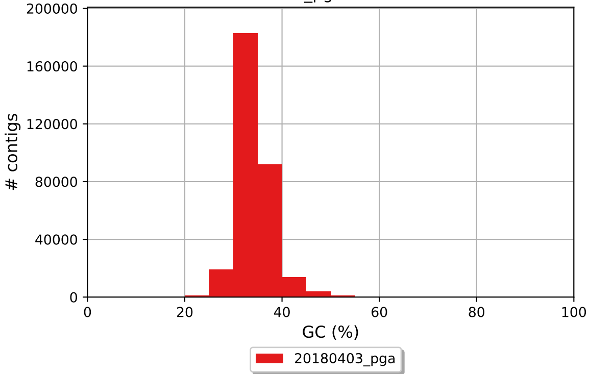
20180403_pga GC content
