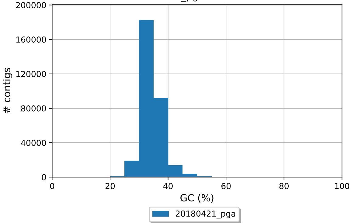
20180421_pga GC content
