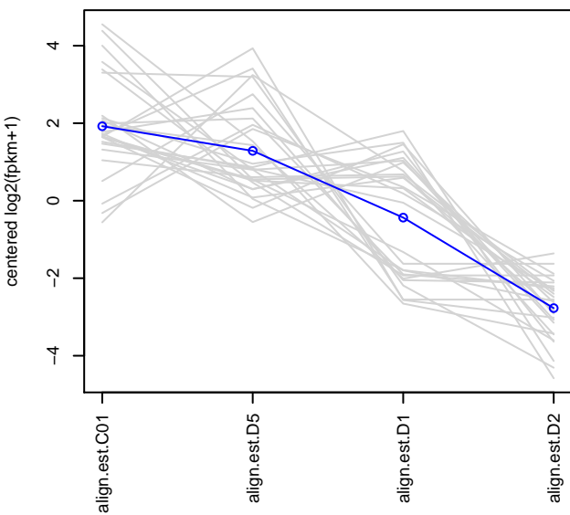
subcluster_5_log2_medianCentered_fpkm.matrix, 27 tra
