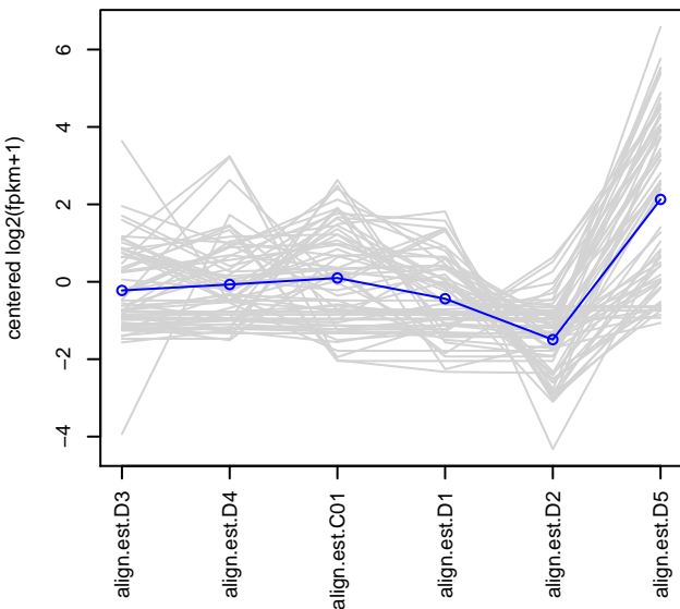
subcluster_10_log2_medianCentered_fpkm.matrix, 62 tra
