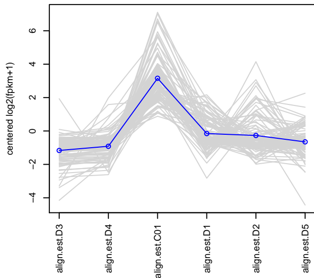
subcluster_3_log2_medianCentered_fpkm.matrix, 103 tra
