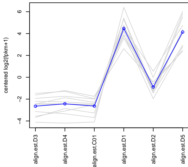
subcluster_11_log2_medianCentered_fpkm.matrix, 11 tra
