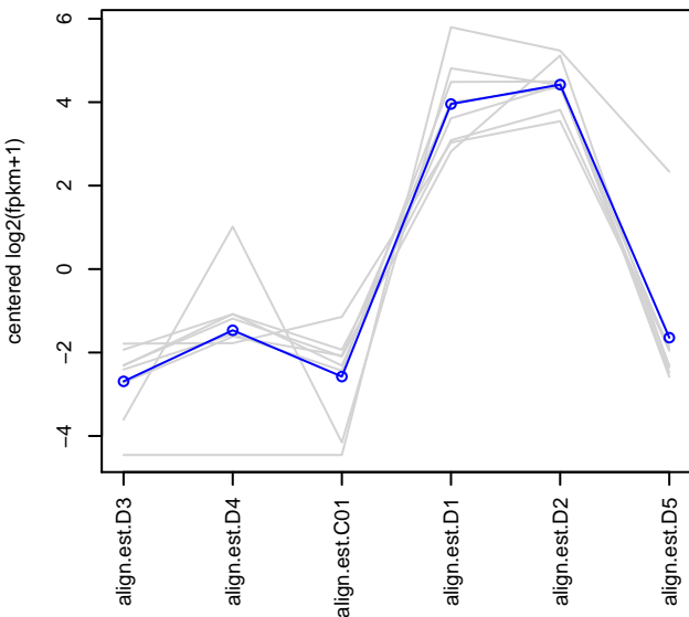
subcluster_12_log2_medianCentered_fpkm.matrix, 8 tra
