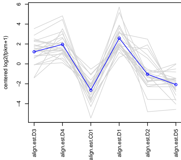
subcluster_1_log2_medianCentered_fpkm.matrix, 24 tra
