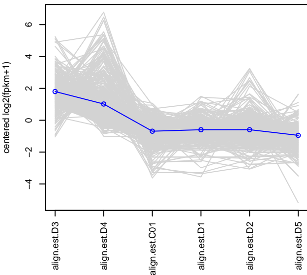
subcluster_2_log2_medianCentered_fpkm.matrix, 428 tra
