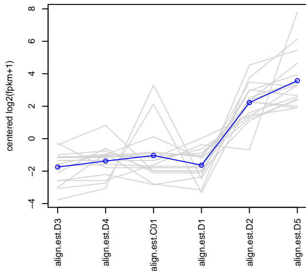
subcluster_5_log2_medianCentered_fpkm.matrix, 16 tra
