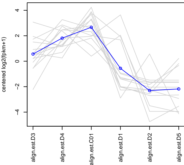
subcluster_4_log2_medianCentered_fpkm.matrix, 14 tra
