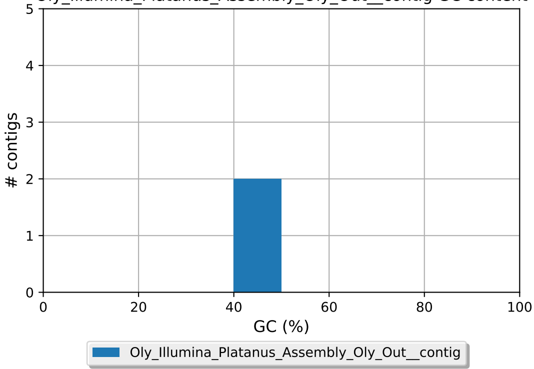
Oly_Illumina_Platanus_Assembly_Oly_Out_contig GC content
