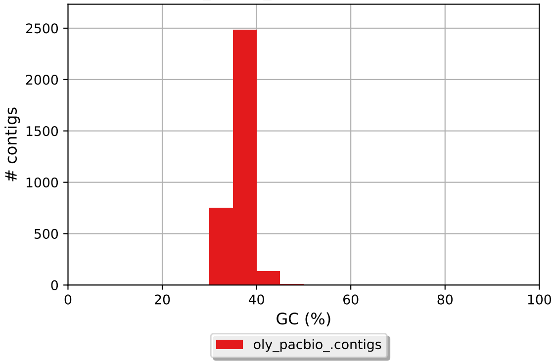
oly_pacbio_.contigs GC content
