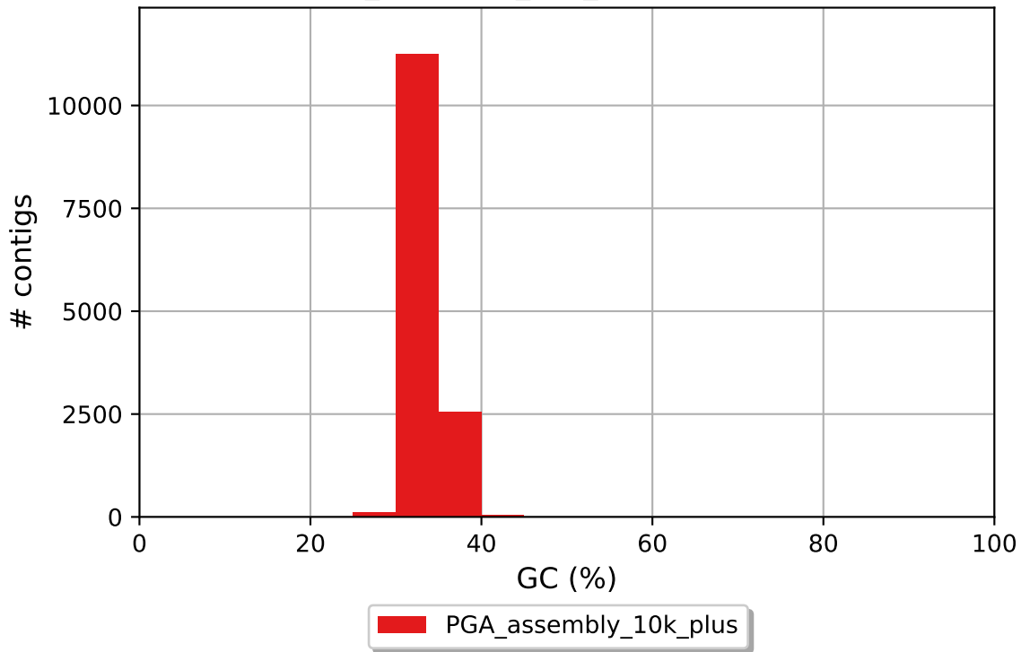
PGA_assembly_10k_plus GC content
